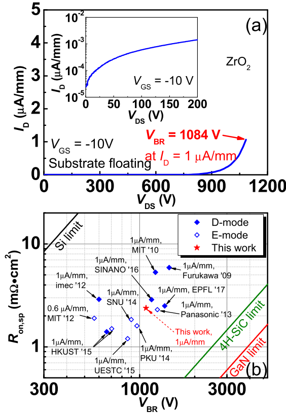
Fig. 7. (a) OFF-state drain leakage current versus drain bias. Inset: semilog plot of I_{DS} for V_{DS} under 200 V. (b) Benchmarking of R_{ON,sp} versus V_{BR} of GaN MOSHEMTs in this paper with the state-of-the-art GaN E/D-mode (MOS)HEMTs on Si by defining V_{BR} at I_{OFF} \leq 1 \mu\text{A/mm} .
