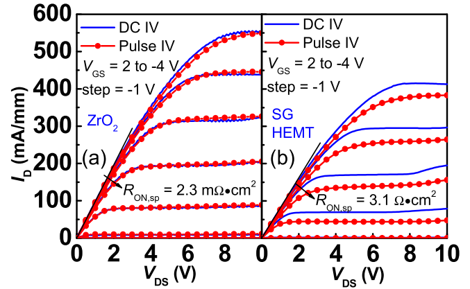
Fig. 6. Comparison of dc and gate-pulsed output characteristics of (a) ZrO 2 -gated MOSHEMTs and (b) SG HEMTs.
