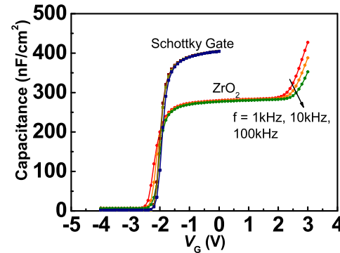
Fig. 3. Multifrequency C – V characteristics of circular-shaped MOS diodes with \text{ZrO}_2 gate dielectric and SG.
