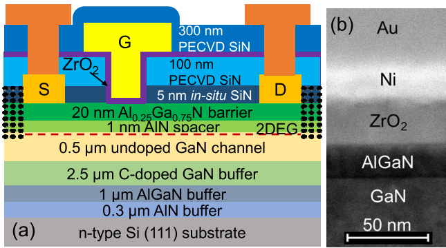
Fig. 1. (a) Cross-sectional schematic of fabricated GaN MOSHEMTs on Si with a 28-nm \text{ZrO}_2 gate dielectric. (b) Cross-sectional TEM image of the gate stack.
