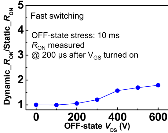
Fig. 8. Dynamic R_{ON} over static R_{ON} ratio as a function of OFF-state drain bias. The substrate was floating during the measurement.
