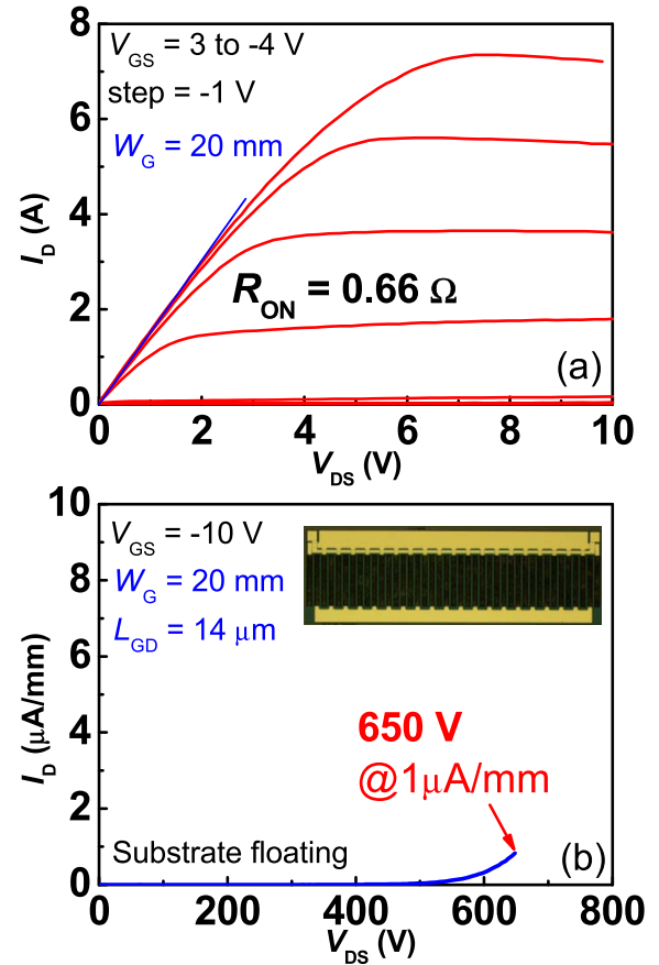
Fig. 9. (a) Output characteristics and (b) OFF-state leakage current of large-area GaN MOSHEMTs with 20-mm gate width. The inset in (b) shows the top-view optical microscope image of the large-area device.
