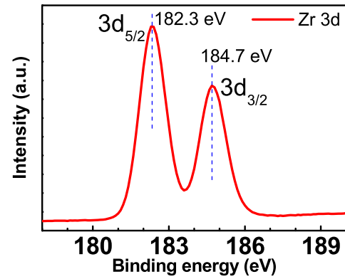
Fig. 2. XPS spectrum of Zr 3d core level of 28-nm \text{ZrO}_2 on AlGaIn/GaN HEMT on Si.
