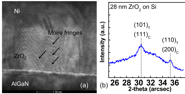
Fig. 4. (a) Cross-sectional TEM image of the ZrO 2 in this paper. (b) XRD pattern of 28-nm ZrO 2 on Si.
