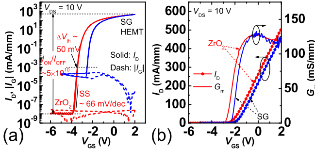
Fig. 5. Comparison of transfer characteristics of MOSHEMTs with ZrO 2 gate dielectric and HEMT with SG (a) in semilog scale and (b) linear scale.
