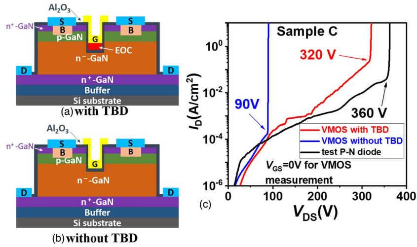
Fig. 4. (Color online) Device schematics of trench MOSFETs (a) with TBD and (b) without TBD. (c) OFF-state I_d - V curves of trench MOSFETs with and without TBD and the trial p-n diode on sample C.
