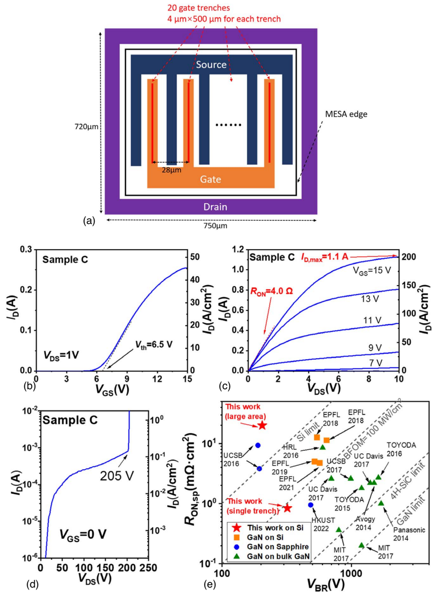
Fig. 5. (Color online) (a) Top-view layout of the large-area trench MOSFET with multiple-finger design. (b) Transfer, (c) output, and (d) OFF-state I_d - V curves of the large-area vertical MOSFET on sample C. (e) R_{ON,sp} versus V_{BR} benchmarking of the GaN-on-Si trench MOSFETs in this work with other reported GaN vertical transistors.
