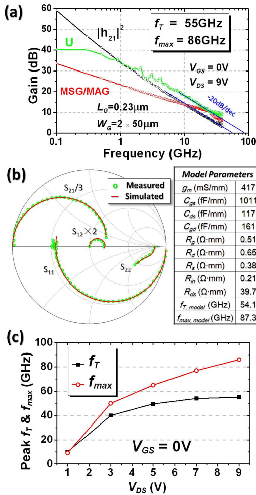
Fig. 8. (a) Small signal RF characteristics of the MISHEMT with L_G = 0.23 \mu\text{m} and W_G = 2 \times 50 \mu\text{m} showing peak f_T/f_{max} of 55/86 GHz. (b) Smith chart of measured and simulated RF data and the table with the model parameters for the device. (c) f_T and f_{max} as a function of V_{DS} for the MISHEMT with L_G = 0.23 \mu\text{m} and W_G = 2 \times 50 \mu\text{m} .
