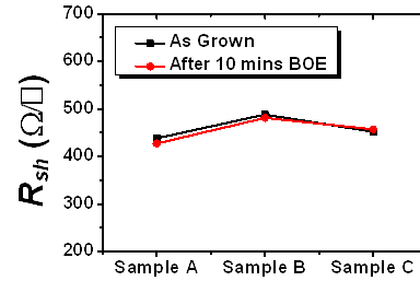
Fig. 4. Sheet resistance R_{sh} of the in situ SiN x /AlN/GaN MISHEMT sample before and after BOE immersion.
