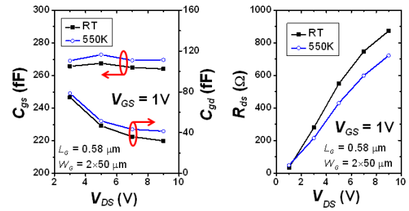
Fig. 12. Thermal dependences of C_{\text{gs}} , C_{\text{gd}} , and R_{\text{ds}} as a function of V_{\text{DS}} .
