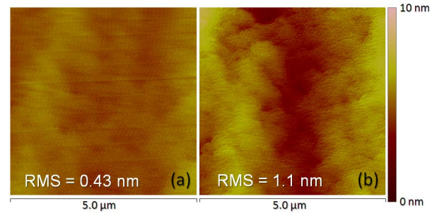
Fig. 1. AFM images of two in situ SiN x /AlN/GaN MISHEMT samples with (a) optimum and (b) nonoptimal in situ SiN x growth conditions.
