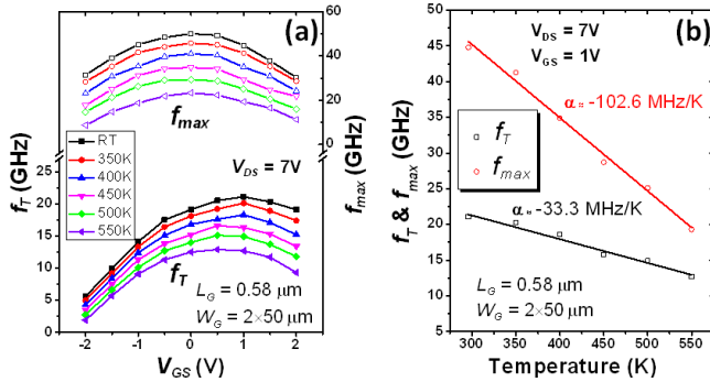
Fig. 11. (a) Thermal evolutions of f_T and f_{\text{max}} as a function of V_{\text{GS}} at V_{\text{DS}} = 7 \text{ V} . (b) Dependences of f_T and f_{\text{max}} on the ambient temperature at V_{\text{GS}} = 1 \text{ V} at V_{\text{DS}} = 7 \text{ V} .
