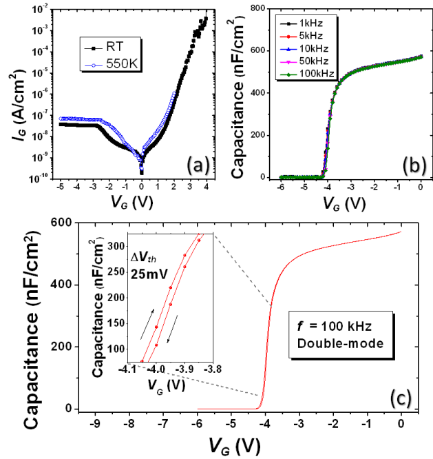
Fig. 2. (a) Gate leakage current measurements of the in situ SiN x /AlN/GaN MIS diode at two different temperatures, RT and 550 K. (b) C - V characteristics of the MIS diode at multiple frequencies. (c) Double-mode C - V characteristics at 100 kHz.
