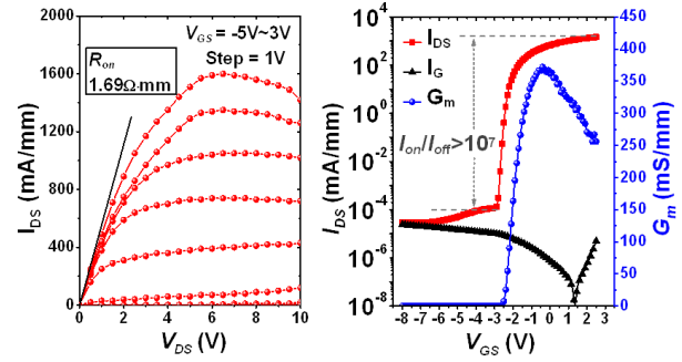
Fig. 6. DC output and transfer characteristics of the MISHEMT with L_G = 0.23 \mu\text{m} and W_G = 2 \times 50 \mu\text{m} .
