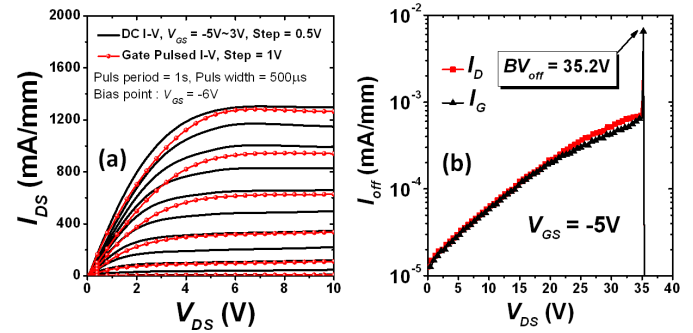
Fig. 7. (a) Gate pulsed and dc output characteristics of the MISHEMT with L_G = 0.58 \mu\text{m} and W_G = 50 \mu\text{m} . (b) Three-terminal OFF-state breakdown characteristics of the MISHEMT at V_{GS} = -5 \text{ V} .
