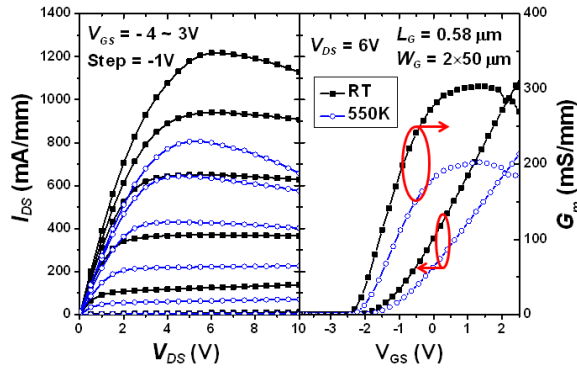
Fig. 10. DC output and transfer characteristics of the MISHEMT with L_G = 0.58 \mu\text{m} and W_G = 2 \times 50 \mu\text{m} at RT and 550 K.
