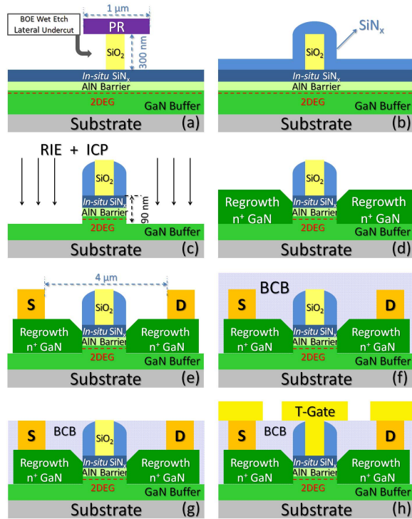
Fig. 3. Schematic of the gate-last self-aligned process flow.
