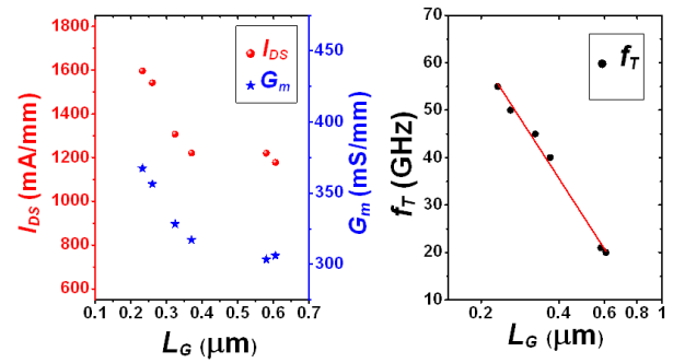
Fig. 9. Scaling behavior of I_{DS} , G_m , and f_T with respect to L_G for the self-aligned gate-last MISHEMTs.
