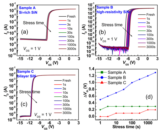
FIG. 4. Monitored transfer characteristics of MISHEMTs of (a) sample A, (b) sample B, and (c) sample C during the forward gate bias stress of +4 V. (d) Measured V_{\text{th}} shift during the gate stress.
