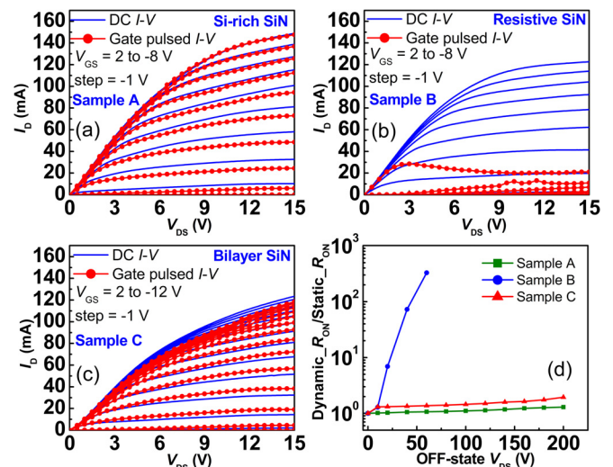
FIG. 2. (a)–(c) Comparison of dc and gate pulsed output characteristics of MISHEMTs of sample A, B, and C. (d) Dynamic- to static- R_{ON} ratio under different off-state drain voltages.
