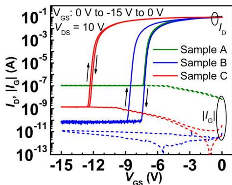
FIG. 1. Double-sweep transfer characteristics of MISHEMTs of sample A (Si-rich), B (high-resistivity), and C (bilayer).
