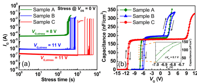
FIG. 3. (a) TDDB gate current monitored on seven MISHEMTs for each of the three samples at room temperature and (b) comparison of double-sweep C - V curves at 1 kHz of MIS diodes of samples A, B, and C. The inset shows the enlarged view of hysteresis in the C - V curve near the pinch-off region of sample A.
