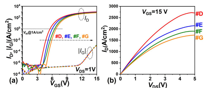
FIG. 3. (a) I_D , |I_G| - V_{GS} (at V_{DS} = 1 V) and (b) I_D - V_{DS} (at V_{GS} = 15 V) curves of samples D, E, F, and G (two-step graded-doped channel with different thickness distributions of high and low doping channels).
