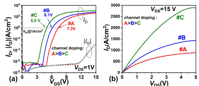
FIG. 2. (a) I_D , |G| - V_{GS} (at V_{DS} = 1 V) and (b) I_D - V_{DS} (at V_{GS} = 15 V) curves of samples A, B, and C (uniformly doped channel with different channel doping concentrations).
