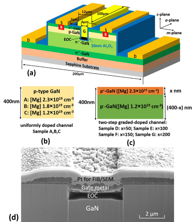
FIG. 1. (a) 3D cross-sectional schematic of fabricated quasi-vertical GaN trench MOSFETs. “S,” “D,” “G,” and “B” refer to “source,” “drain,” “gate,” and “body,” respectively. Ethylene octene copolymer (EOC) at the gate trench is used as bottom dielectric to manage the electric field. p-type GaN epi infomation of (b) uniformly doped channel (samples A, B, and C); (c) step-graded channel (samples D, E, F, and G). (d) Cross-sectional SEM image of the gate trench region of a fabricated device.
