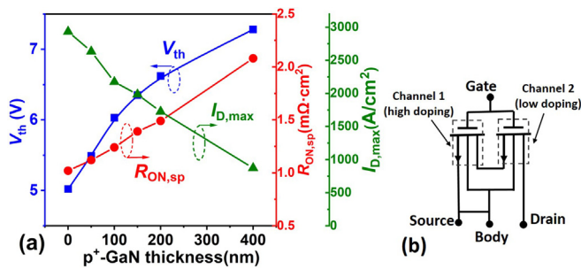
FIG. 4. (a) Experimental values of R_{ON,sp} , I_{D,max} , and V_{th} vs p^+-GaN layer thickness. Data points on p^+-GaN thickness = 0, 50, 100, 150, 200, and 400 nm correspond to samples C, D, E, F, G, and A, respectively. (b) Equivalent two-transistor sub-circuit model 25 for step-graded channel.
