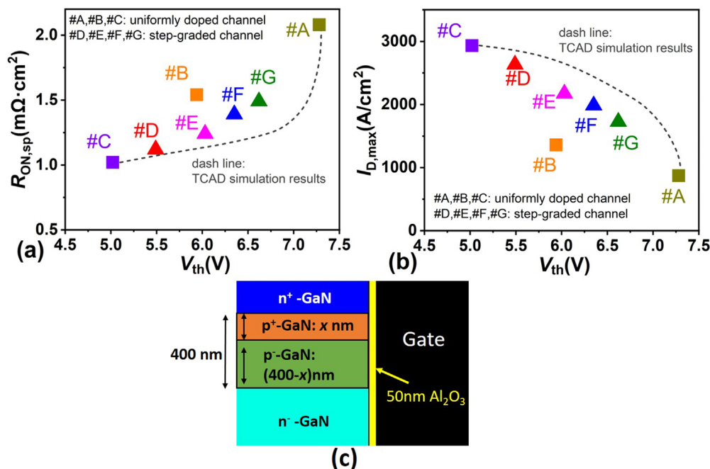
FIG. 5. Experimental results of (a) R_{ON,sp} vs V_{th} and (b) I_{D,max} vs V_{th} of all fabricated seven samples. (c) Simulation structures of device with two-step graded-doped channel. The simulation results are also included in (a) and (b).
