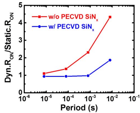
Fig. 12. Dynamic R_{ON} under various pulse periods extracted from Fig. 11.
