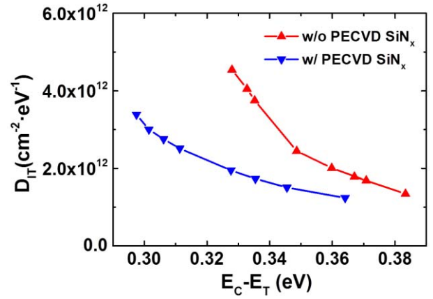
Fig. 10. Interface trap density as a function of the energy level depth below the conduction band for the MIS diodes with and without PECVD \text{SiN}_x passivation.
