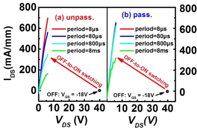
Fig. 11. Transient OFF-to-ON switching measurements under various stress periods from 8 \mu s to 8 ms. The applied pulsewidth is 0.8 \mu s. The MISHEMTs with and without passivation were switched from the off state with a quiescent bias of (V_{GSQ}, V_{DSQ}) = (-18, 40 V) to the ON state with a gate bias of 2 V.
