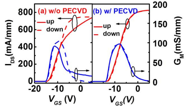
Fig. 3. Double-mode dc transfer curves of LPCVD \text{SiN}_x /AlGaIn/GaN MISHEMTs with and without PECVD \text{SiN}_x passivation ( V_{\text{DS}} = 10 \text{ V} ).
