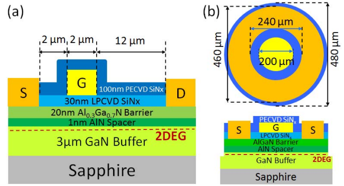
Fig. 2. Schematic diagrams of the LPCVD \text{SiN}_x /AlGaIn/GaN MISHEMT and MIS diode with PECVD \text{SiN}_x passivation.
