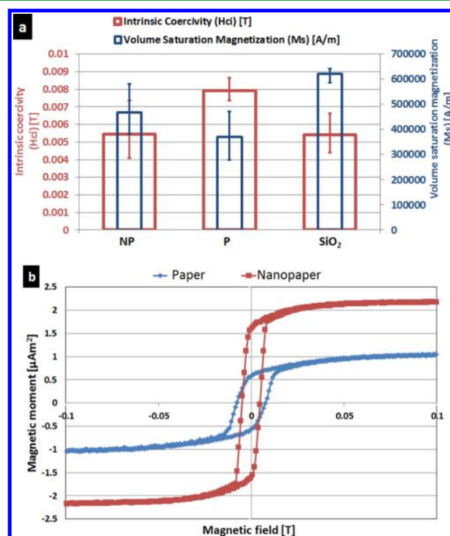
Figure 9. (a) Comparison of the intrinsic coercivity and the saturation magnetization of 150 nm of Py:Ni 81wt% Fe 19wt% sputter deposited onto nanopaper (NP), commercially available paper (P), and silicon dioxide (SiO 2 ) platforms. The error bars in the measurements are mainly due to the slight variation in coating thickness due to the sputter deposition process, and, in the case of the commercial paper surface, also due to the stochastic paper surface. (b) Thin-tall magnetization hysteresis of the nanopaper-based Py:Ni 81wt% Fe 19wt% coating compared to a wider and shorter magnetization hysteresis on regular paper platforms.
