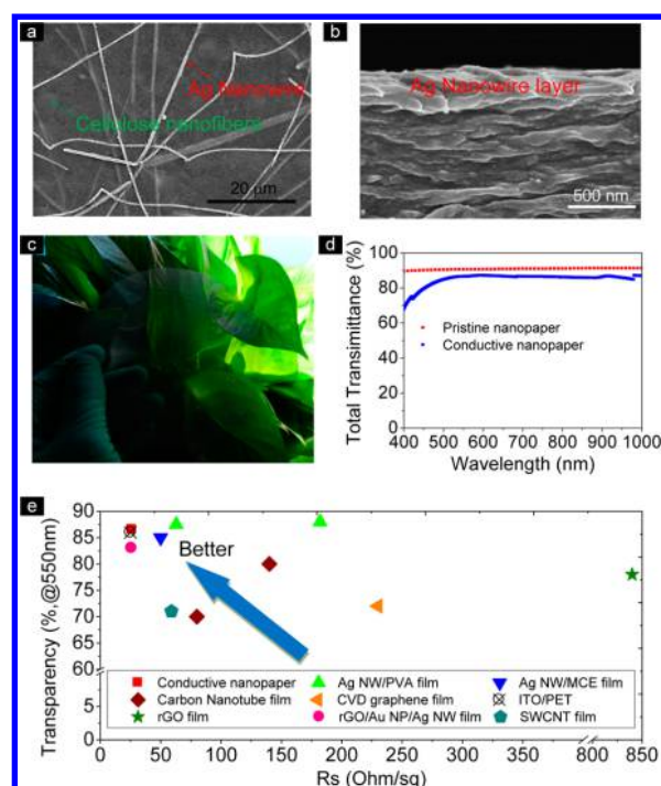
Figure 5. Top view SEM images of the (a) surface and (b) cross-section of Ag nanowire coating nanopaper. (c) Digital image to illustrate the optical transparency of Ag nanowire coated nanopaper, which was measured (d) to be 86.5% at 550 nm. (e) Comparative study of optical transparency (at 550 nm) and R_s values of our conductive nanopaper, Ag NW/PVA film, Ag NW/mixed esters of cellulose (MCE) film, carbon nanotube film, CVD graphene film, ITO/PET film, rGO film, rGO/Au NP/Ag NW film, and SWCNT film.
