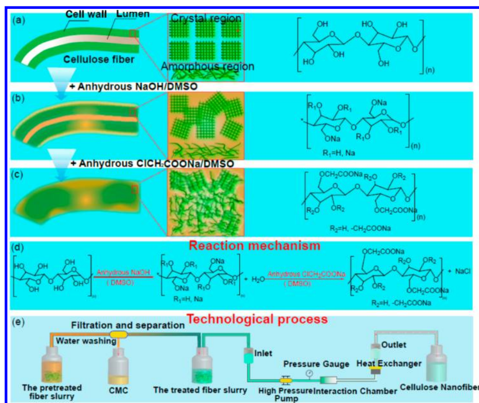
Figure 1. Schematic illustrations of the preparation of cellulose nanofibers by a novel partial dissolution method. (a) Hierarchical and chemical structures of natural wood fiber. (b) Basification of cellulose in anhydrous NaOH/DMSO solution which swells the tight crystal region. (c) Sodium acetoxylation of the basified cellulose fibers by introducing -CH 2 COONa groups into the cellulose. Further washing by water facilitates the separation of cellulose fibers and sodium carboxymethylcellulose (CMC). (d) Reaction mechanisms of basification and sodium acetoxylation of cellulose fibers in anhydrous DMSO environment. (e) Technological process of separating cellulose fibers, homogenization of the pretreated cellulose fiber suspension, and disintegration from the microscopic cellulose fibers into the cellulose nanofibers.
