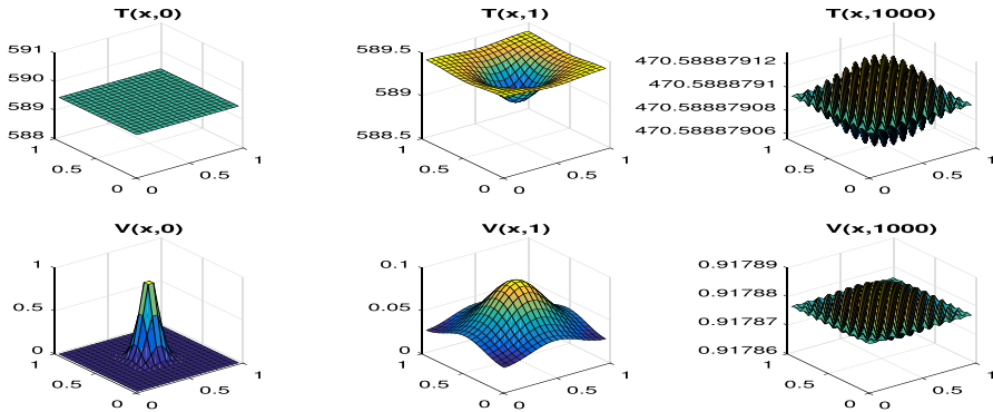
Fig. 1 The CTL-inactivated steady state E_1 is globally asymptotically stable when R_0 > 1 and R_1 < 1
